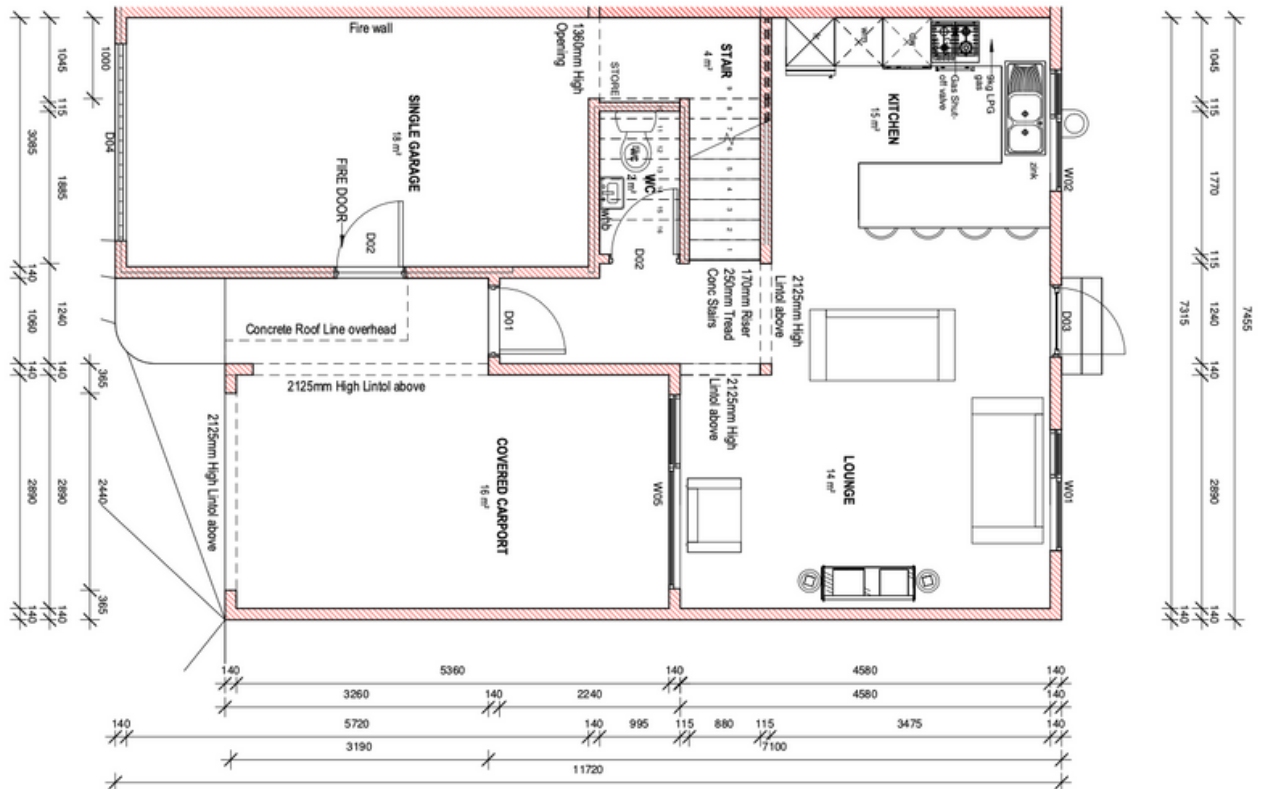
1 1 : 50 GROUND FLOOR PLAN
