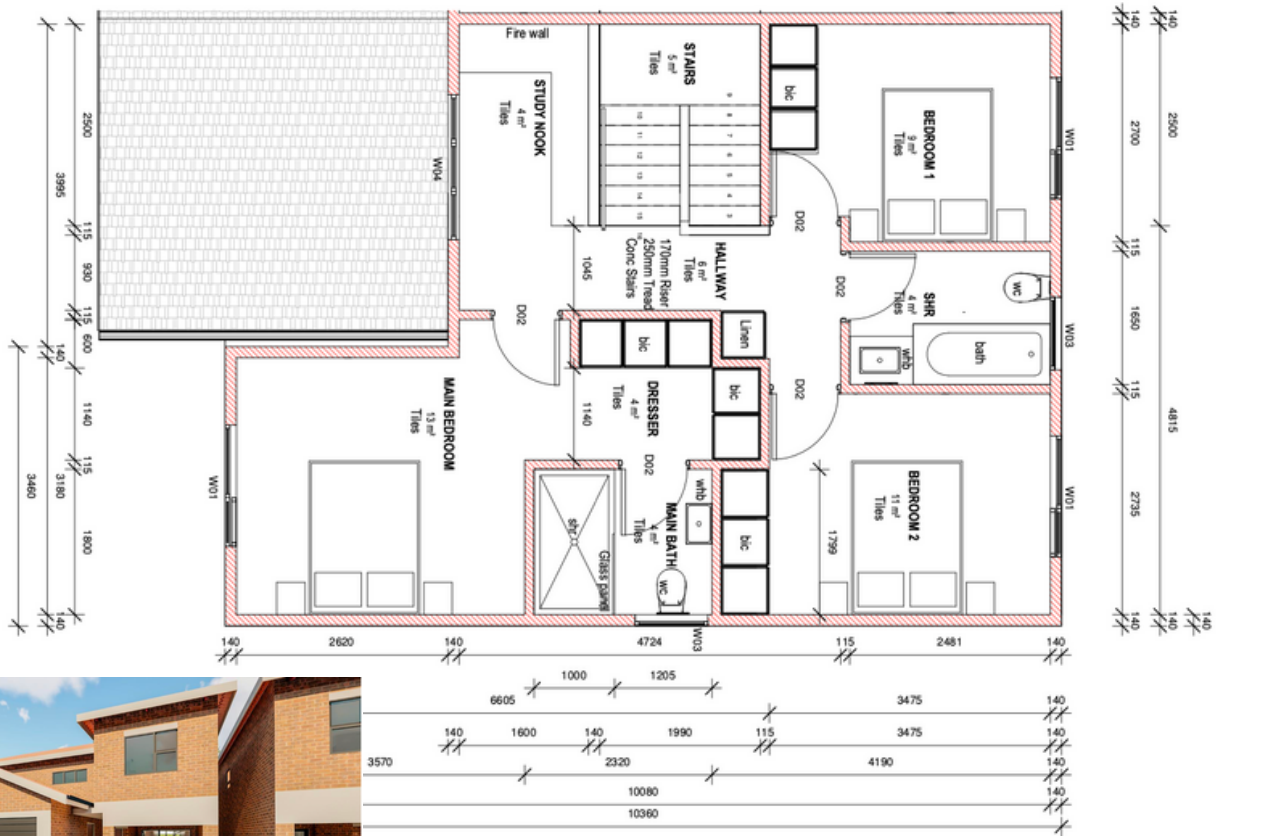
2 1 : 50 FIRST FLOOR PLAN
